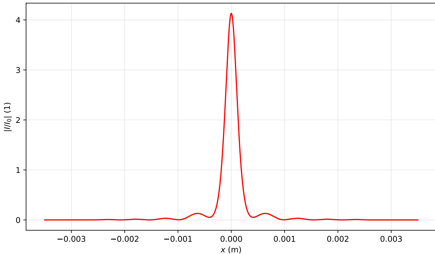
Intensity profile I(x, y = 0, z = 0.478)/I_0 , P_{in}=1.0P_{cr} , artificial time
